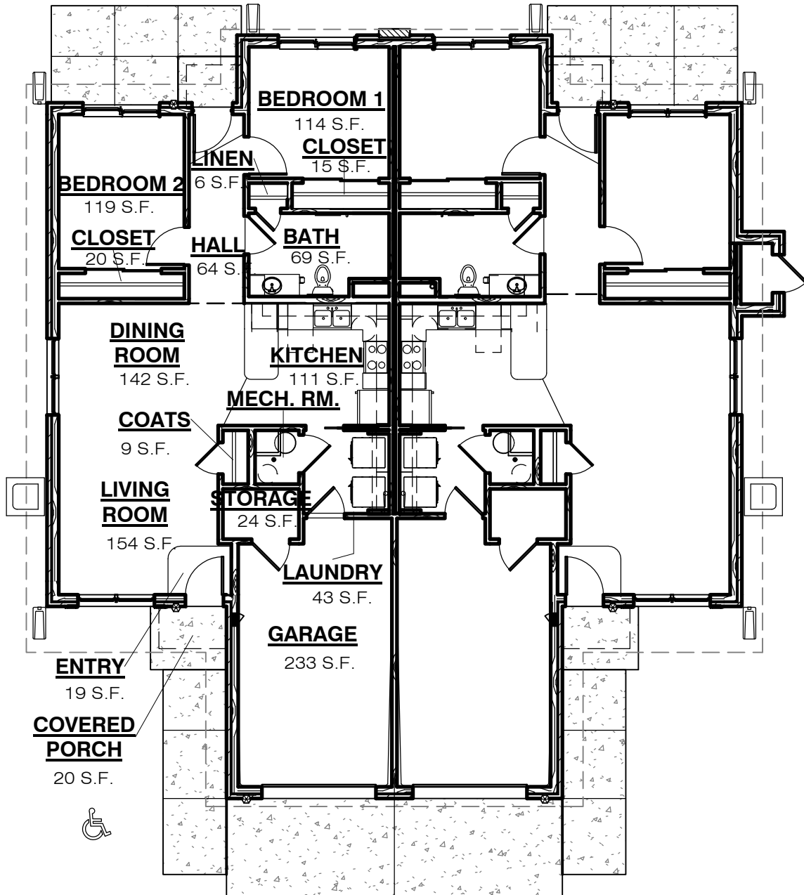
1 KENSINGTON FLOOR PLAN 1064 SF K1 3/32" = 1'-0"
