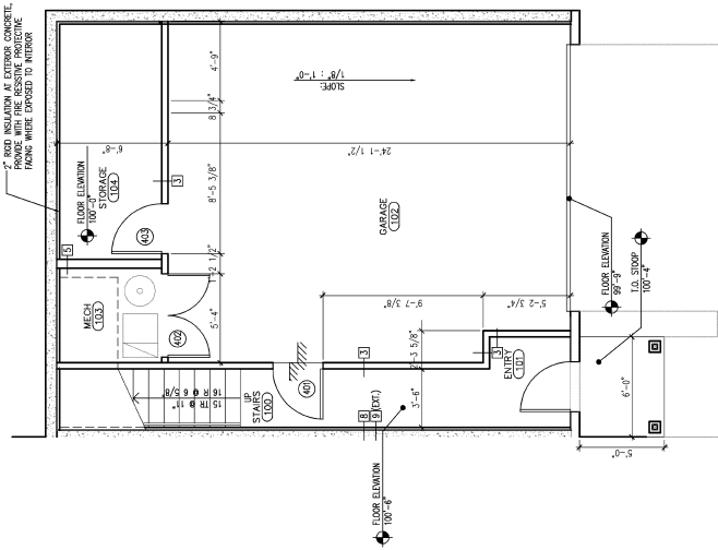
4 Bedroom First Floor Plan SCALE: 1/4" = 1'-0"
