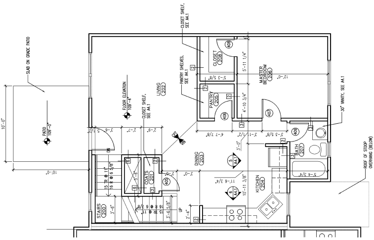
4 Bedroom- Second Floor Plan SCALE: 1/4" = 1'-0"
